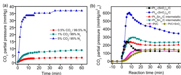
Figure 3. (a) CO 2 microelectrode responses in various CO 2 gas environments. (b) ECASA-specific P_{CO_2} of Pt/Sn and Pt catalysts.
